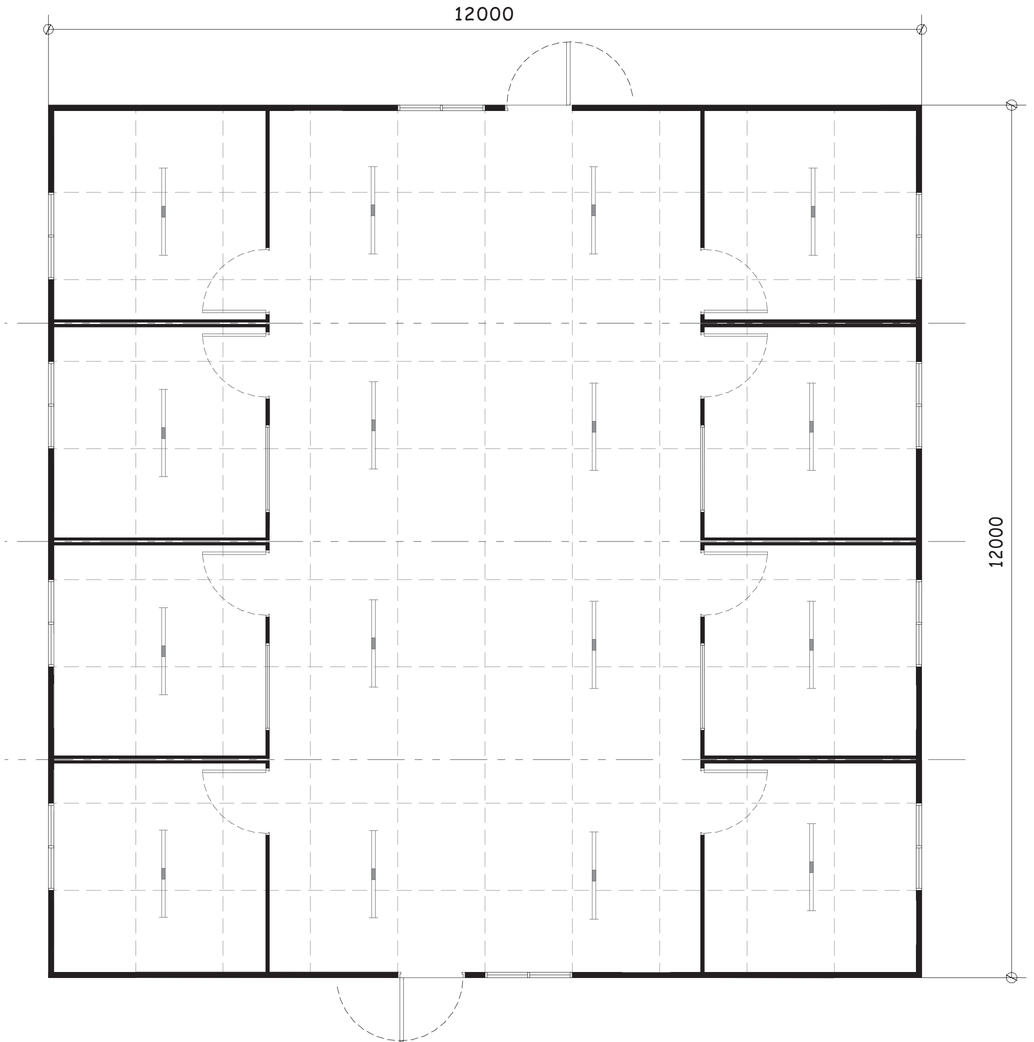
12.0 x 12.0 OFFICE
